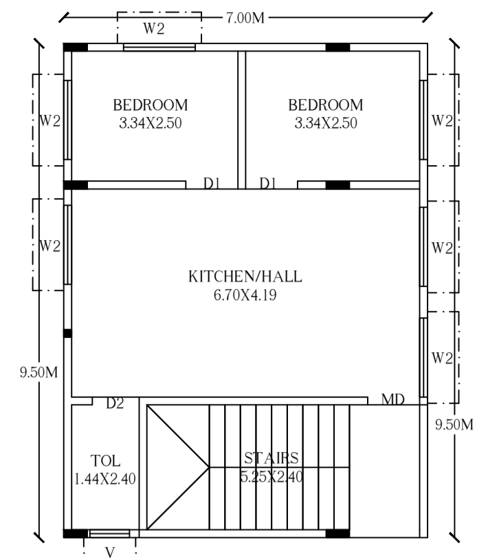
TYPICAL GROUND, FIRST & SECOND FLOOR PLAN
